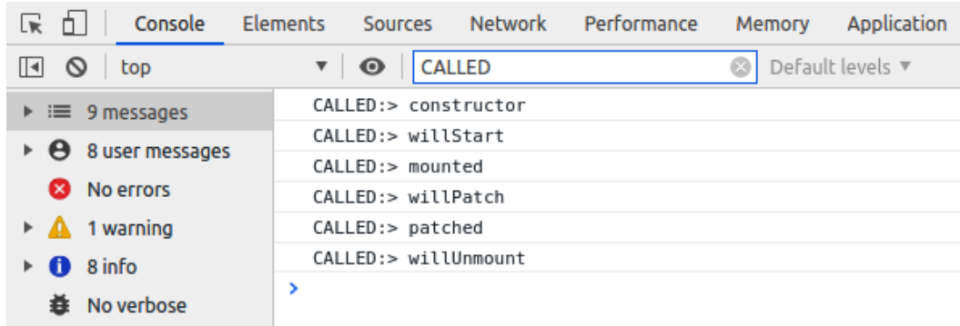
Figure 16.4 – Logs in the browser console
