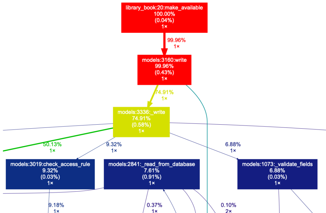
Figure 21.1 – Graph to check execution times
