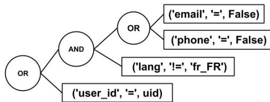
Figure 9.2 – The evaluation of a domain
