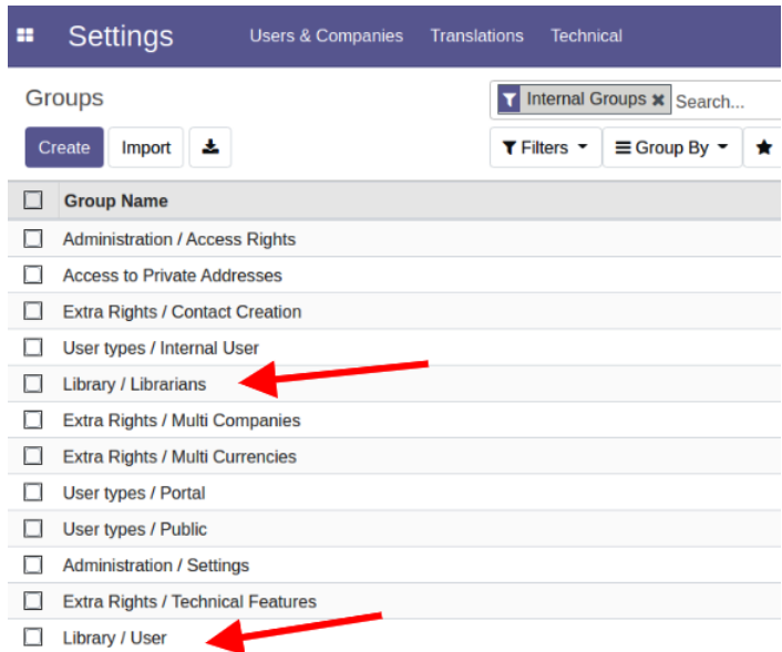
Figure 10.1 – Newly added security groups
