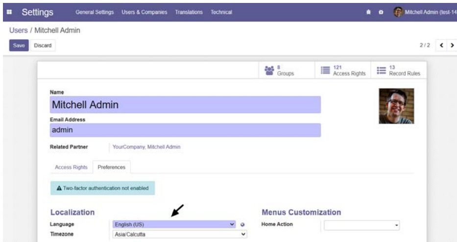
Figure 11.4 – User's form to set the language
