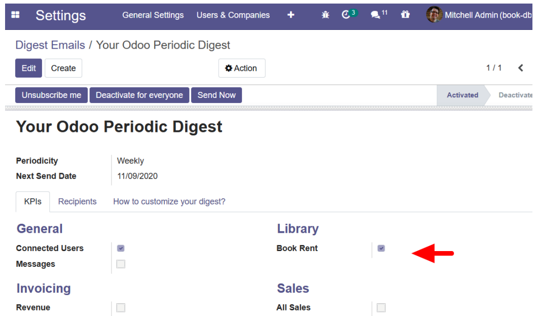
Figure 23.12 – Enabling the digest email for book rent data
