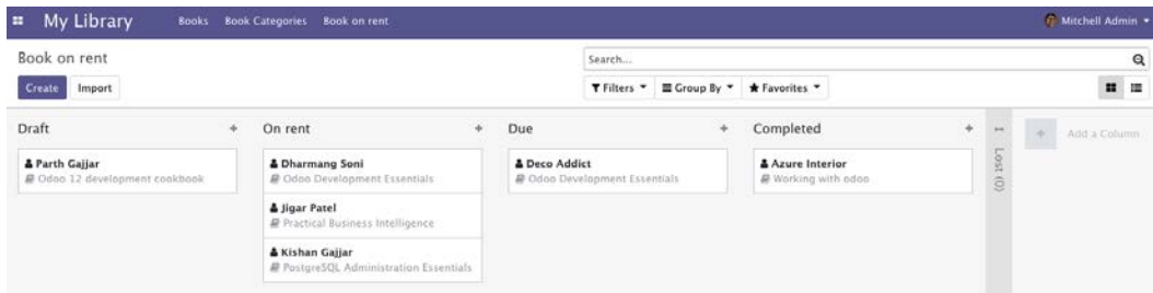
Figure 12.2 – Kanban view with groups by stage
