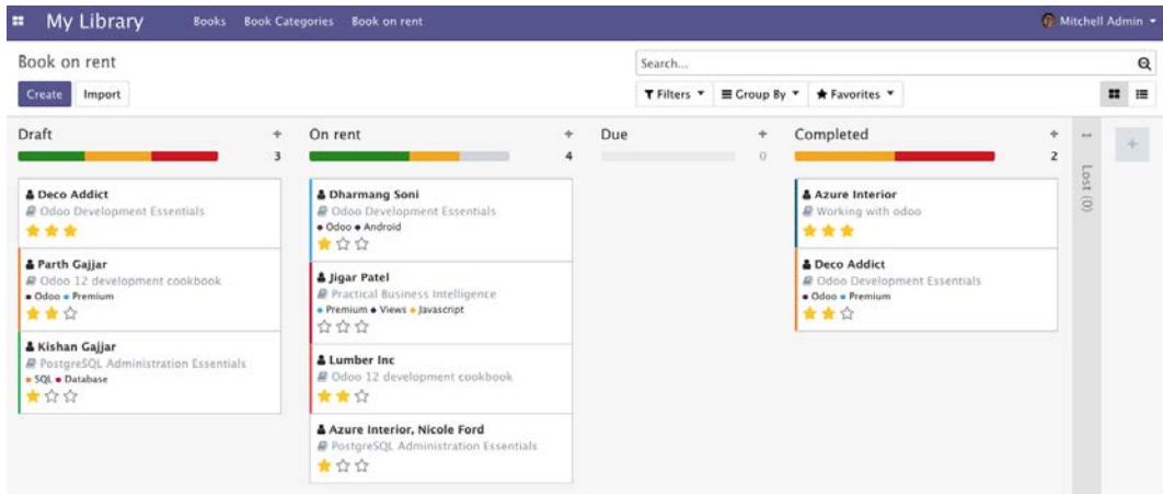
Figure 12.6 – Kanban view with a progress bar
