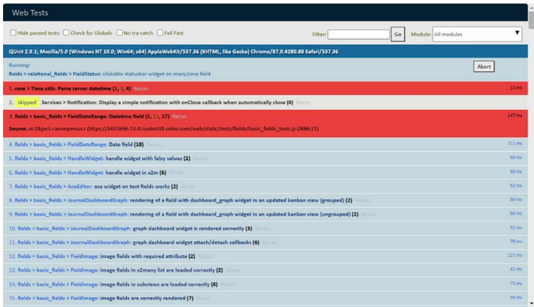
Figure 18.2 – Results of QUnit test cases
