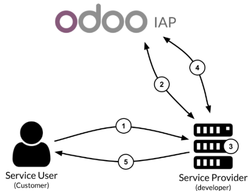
Figure 17.1 – IAP workflow
