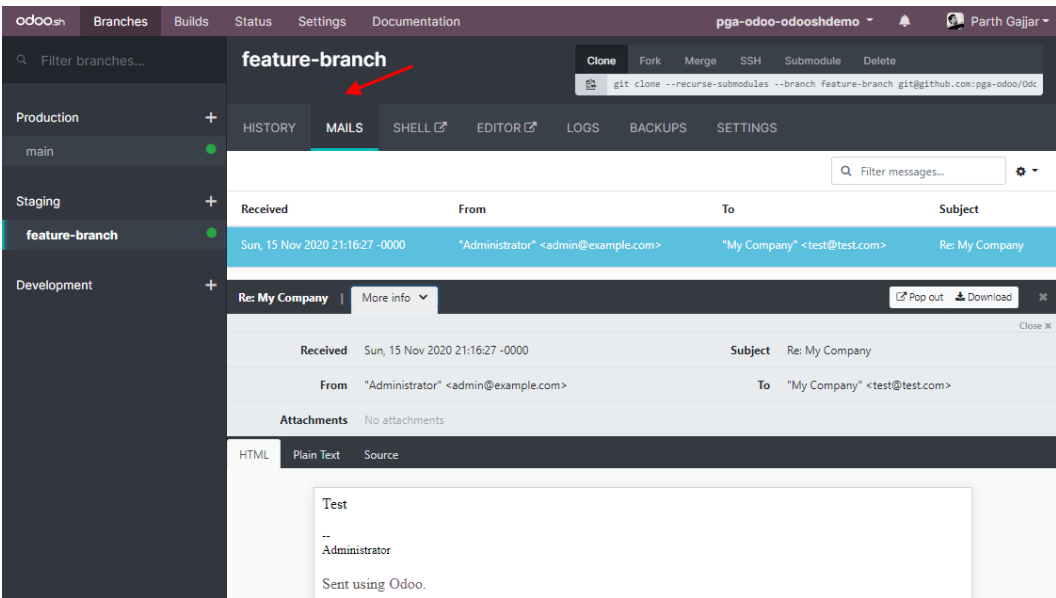
Figure 19.12 – Mail catcher
