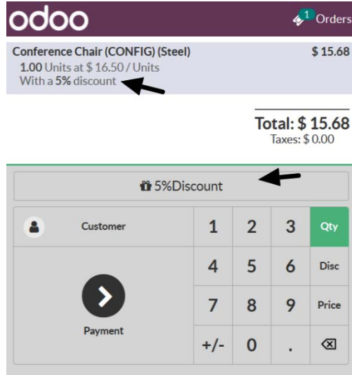
Figure 22.3 – Discount button
