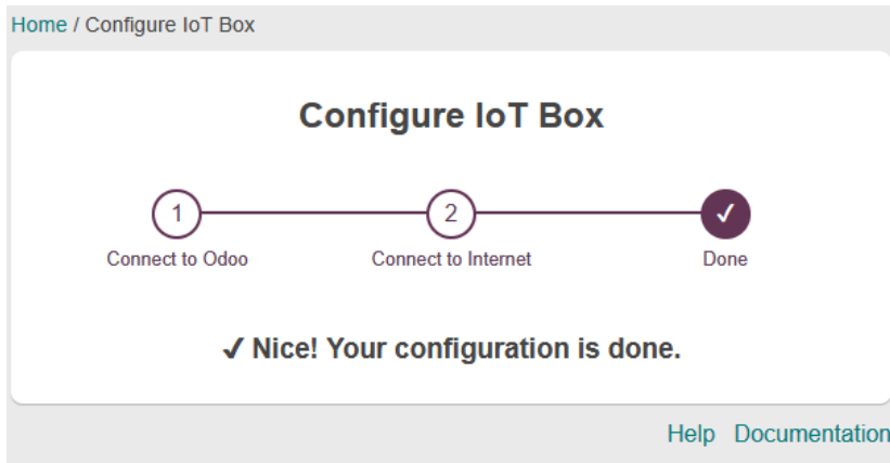
Figure 24.6 – Confirmation page
