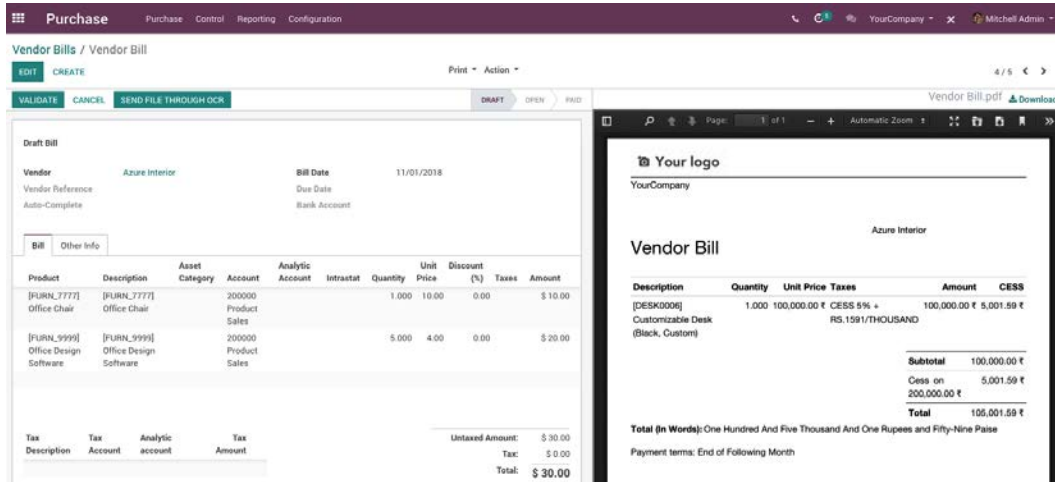
Figure 9.3 – Cascading attachments and the form view
