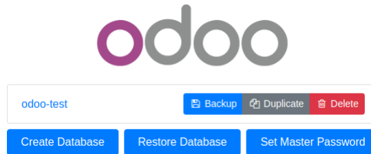
Figure 1.3 – Database manager
