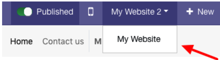
Figure 14.4 – Website switcher
