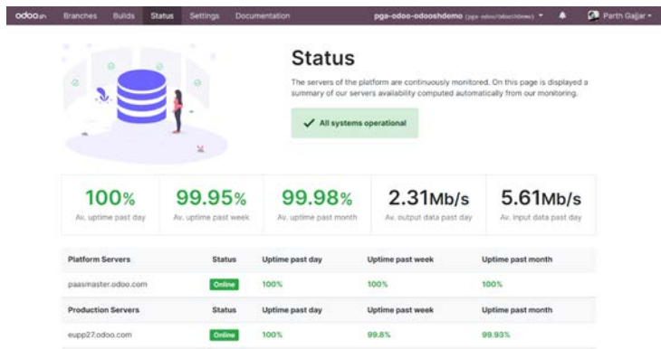
Figure 19.19 – Odoo.sh status
