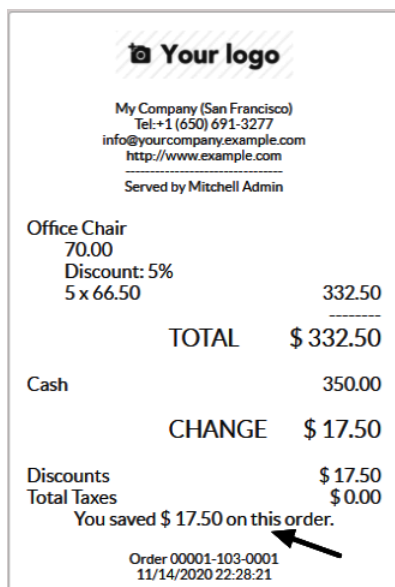
Figure 22.7 – Updated receipt
