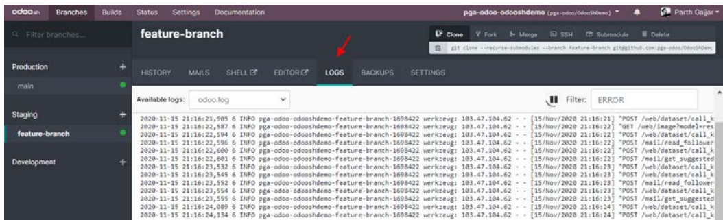
Figure 19.15 – Server log
