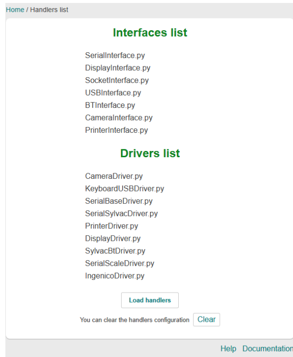
Figure 24.16 – Drivers list
