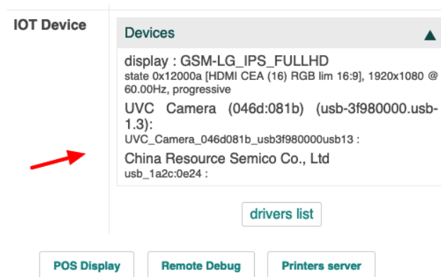
Figure 24.17 – Connected devices
