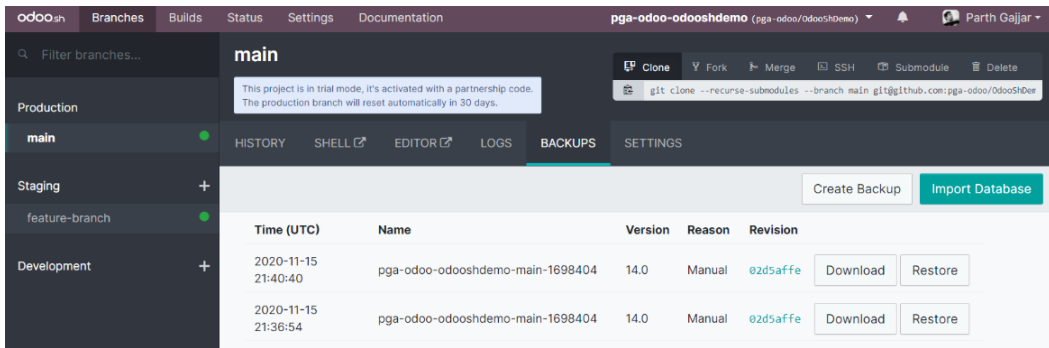
Figure 19.17 – Backups manager
