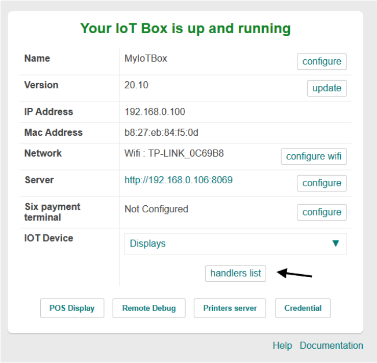
Figure 24.15 – Handlers list
