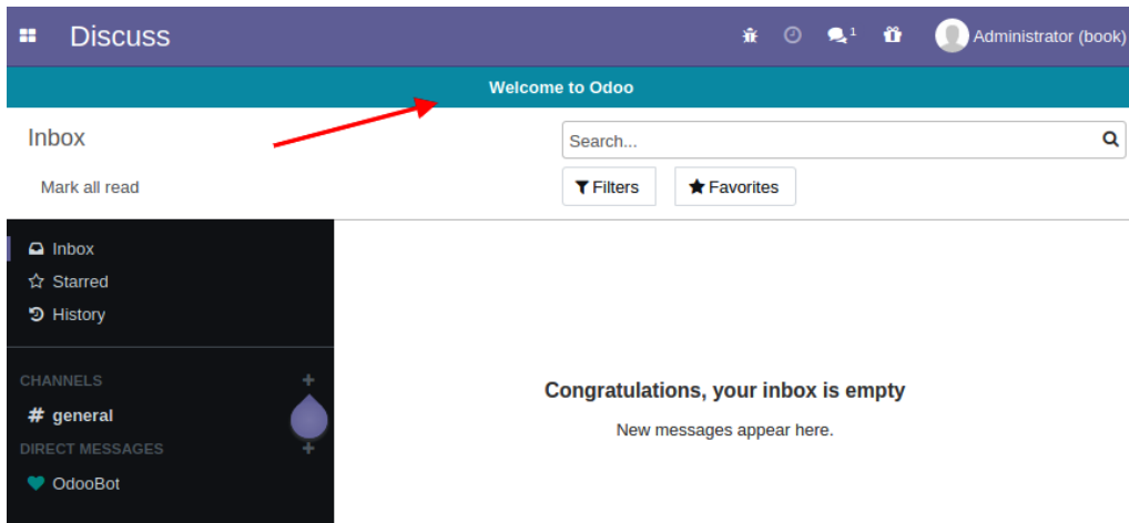
Figure 16.1 – OWL component
