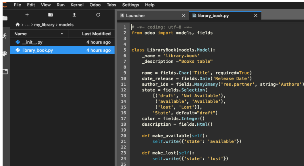
Figure 19.14 – Web code editor
