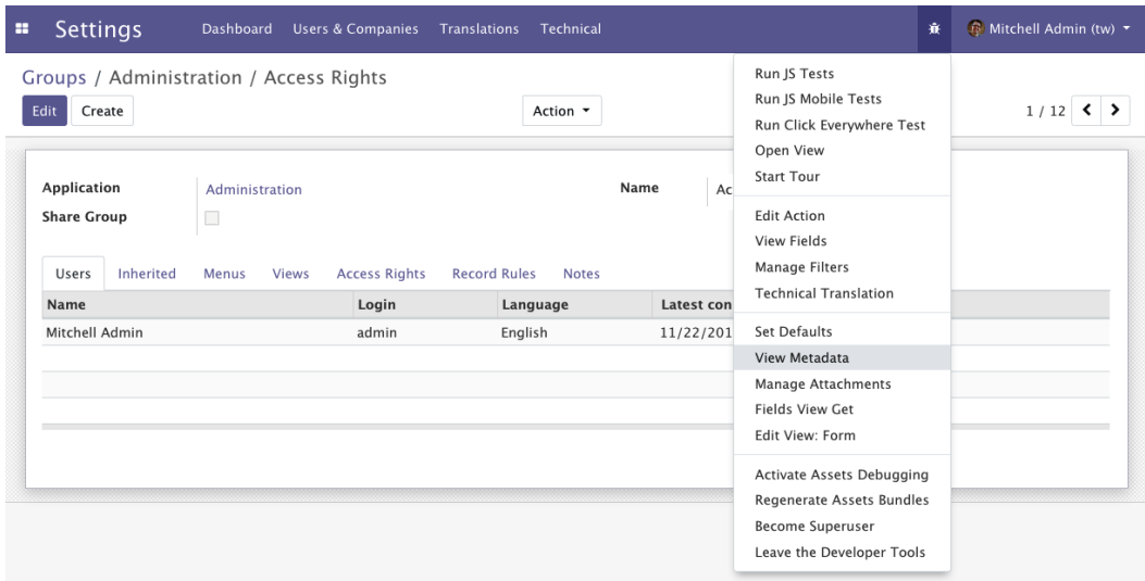
Figure 10.3 – Menu for viewing a group's XML ID
