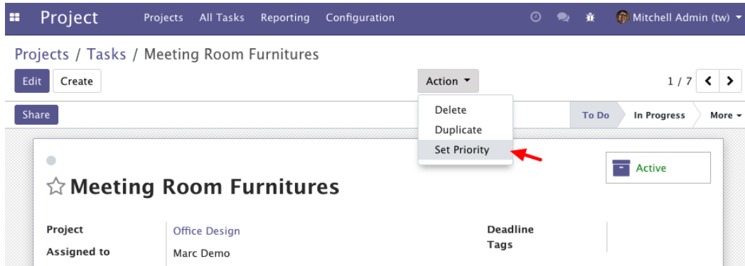
Figure 12.9 – Set Priority server action
