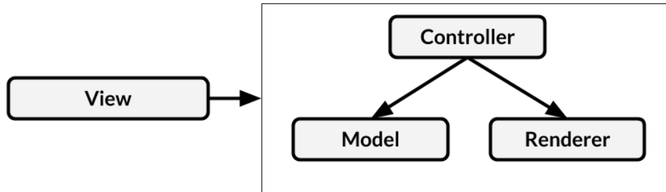
Figure 15.4 – View components
