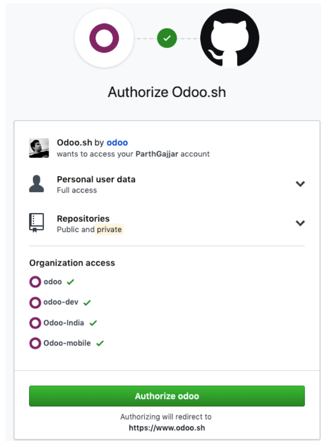
Figure 19.1 – GitHub authentication
