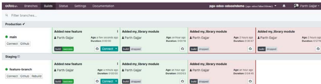
Figure 19.18 – Build status
