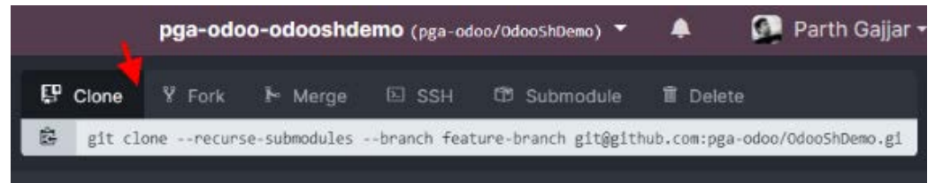
Figure 19.16 – Git commands
