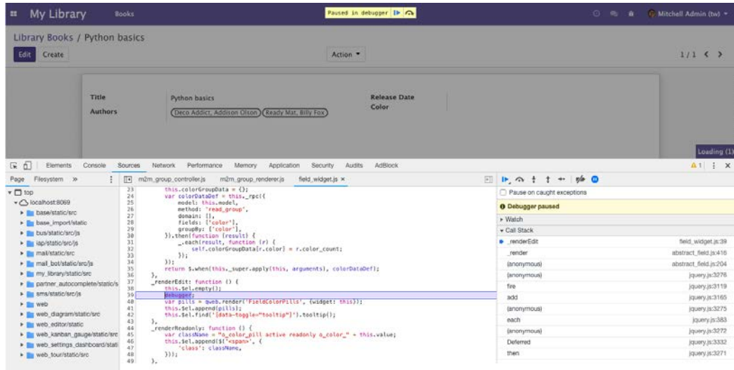
Figure 15.6 – Paused debugger
