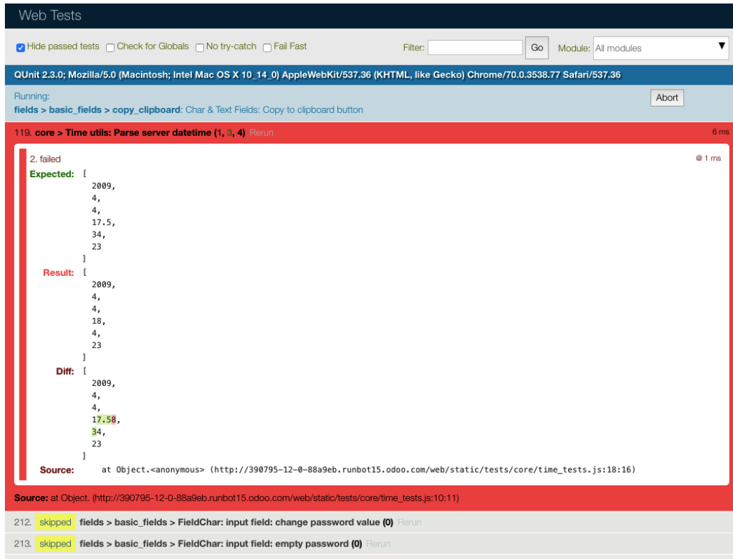
Figure 7.2 – QUnit test case result screen
